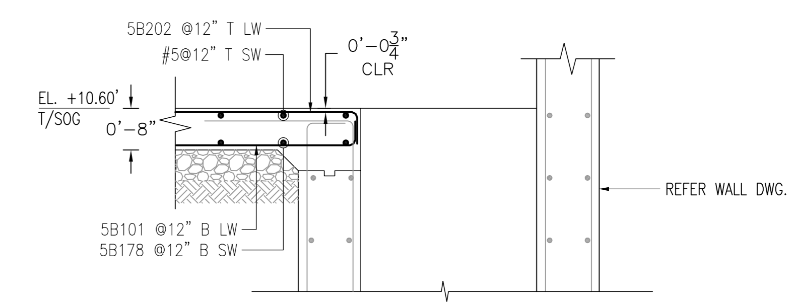
8 SECTION 1/2"=1'-0" SDR: 4/FO-202.00
