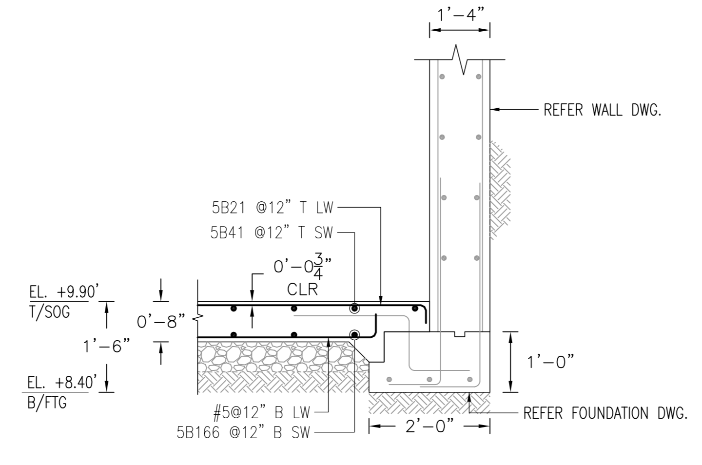
2 SECTION 1/2"=1'-0" SDR: 8/FO-202.00
