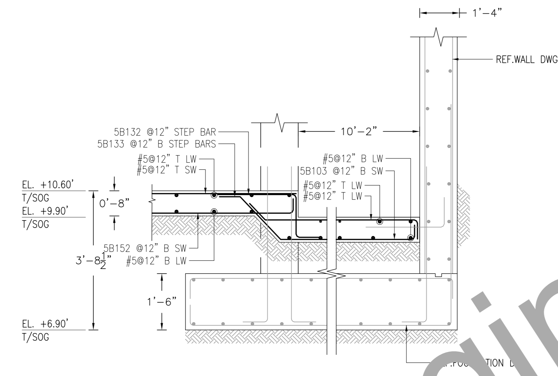
6 SECTION 1/2"=1'-0" SDR: 9/FO-202.00
