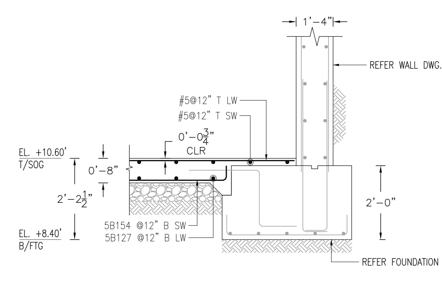
3 SECTION 1/2"=1'-0" SDR: 1A/FO-202.00
