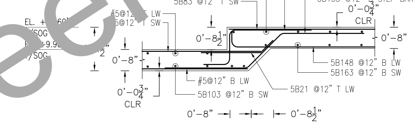
7 SECTION 1/2"=1'-0" SDR: 4/FO-201.00
