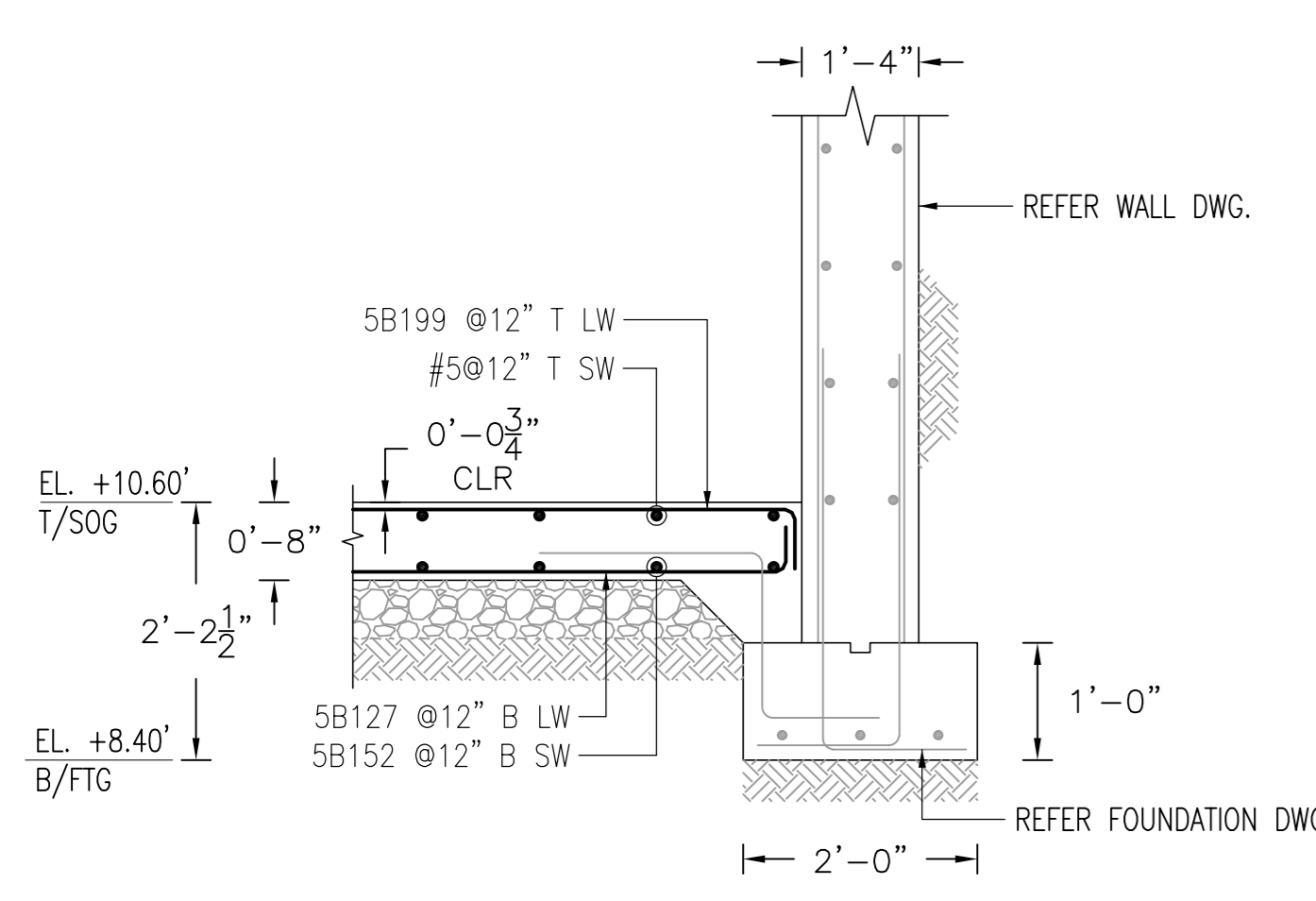
1 SECTION 1/2"=1'-0" SDR: 1/FO-202.00
