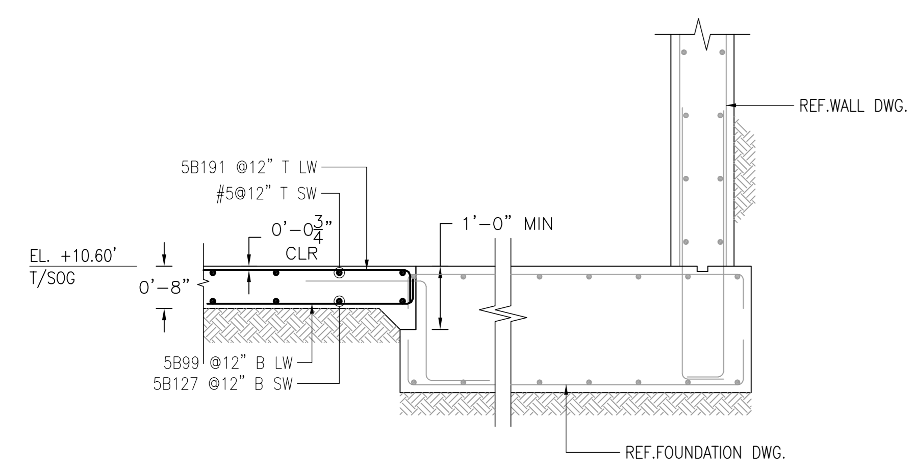
5 SECTION 1/2"=1'-0" SDR: 3/FO-202.00
